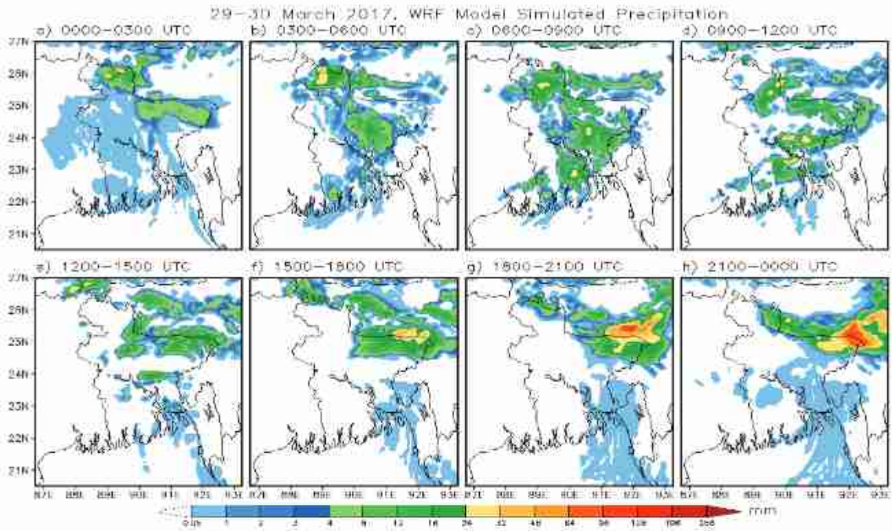
Figure 5: Spatial distribution of simulated 3 hourly accumulated rainfalls over Bangladesh during 28-30 March 2017.
