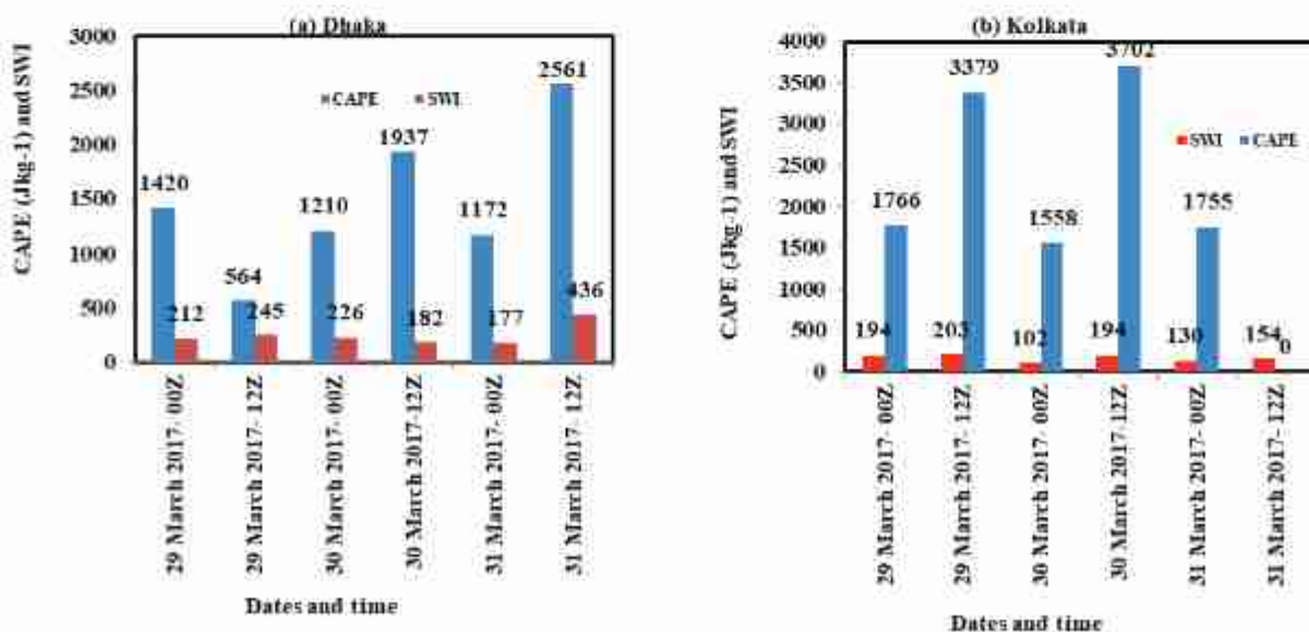
Figure 4: Temporal variation of CAPE and SWI at (a) Dhaka and (b) Kolkata.
