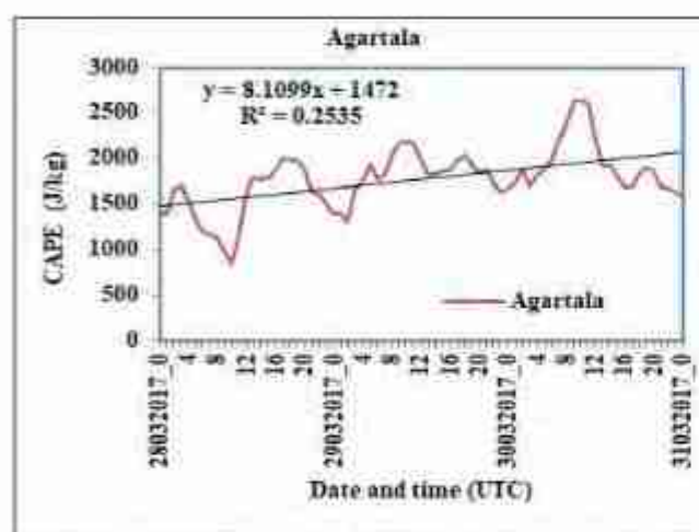
Figure 14: Hourly variation in CAPE at Agartala during 28-31 March 2017.
