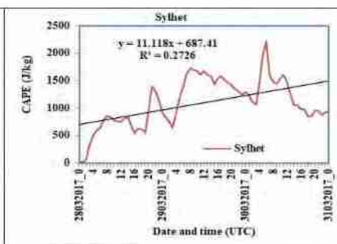
Figure 15: Hourly variation in CAPE at Sylhet during 28-31 March 2017.
