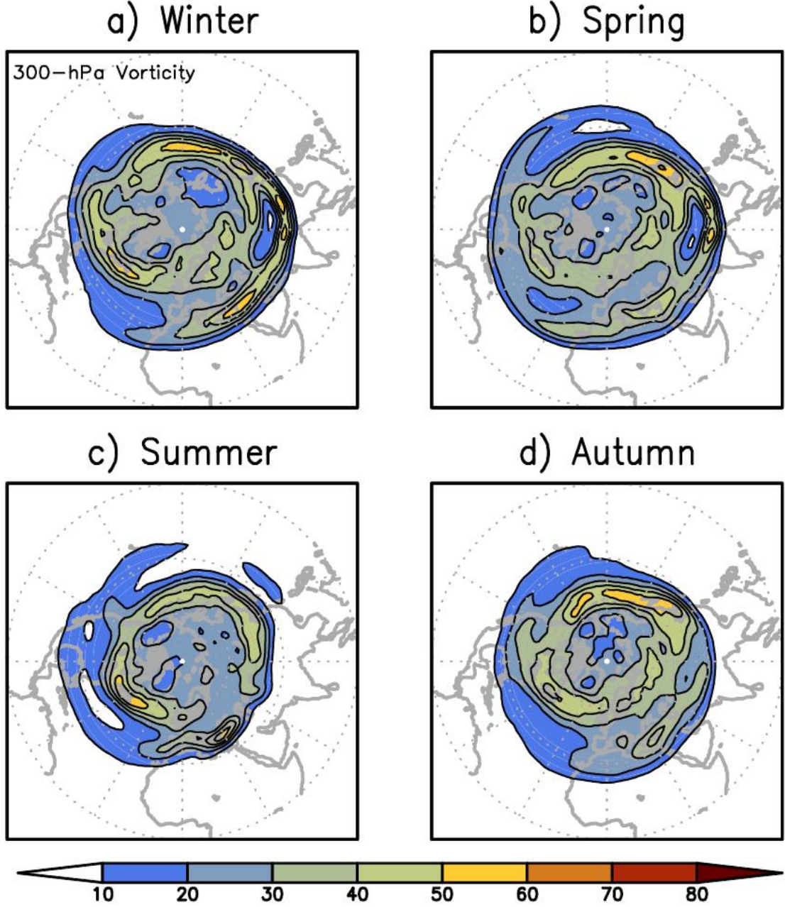
Figure 5: Track density for positive 300-hPa relative vorticity for boreal seasons for the period (1979-2014): a) Winter, b) Spring, c) Summer and d) Autumn. Units are number density per season per unit area where unit area is equivalent to 5^\circ radius spherical cap.
