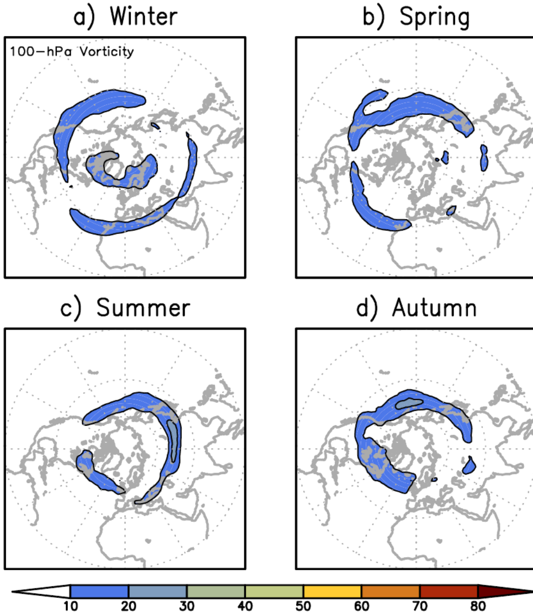
Figure 6: Track density for positive 100-hPa relative vorticity for boreal seasons for the period (1979-2014): a) Winter, b) Spring, c) Summer and d) Autumn. Units are number density per season per unit area where unit area is equivalent to 5^\circ radius spherical cap.
