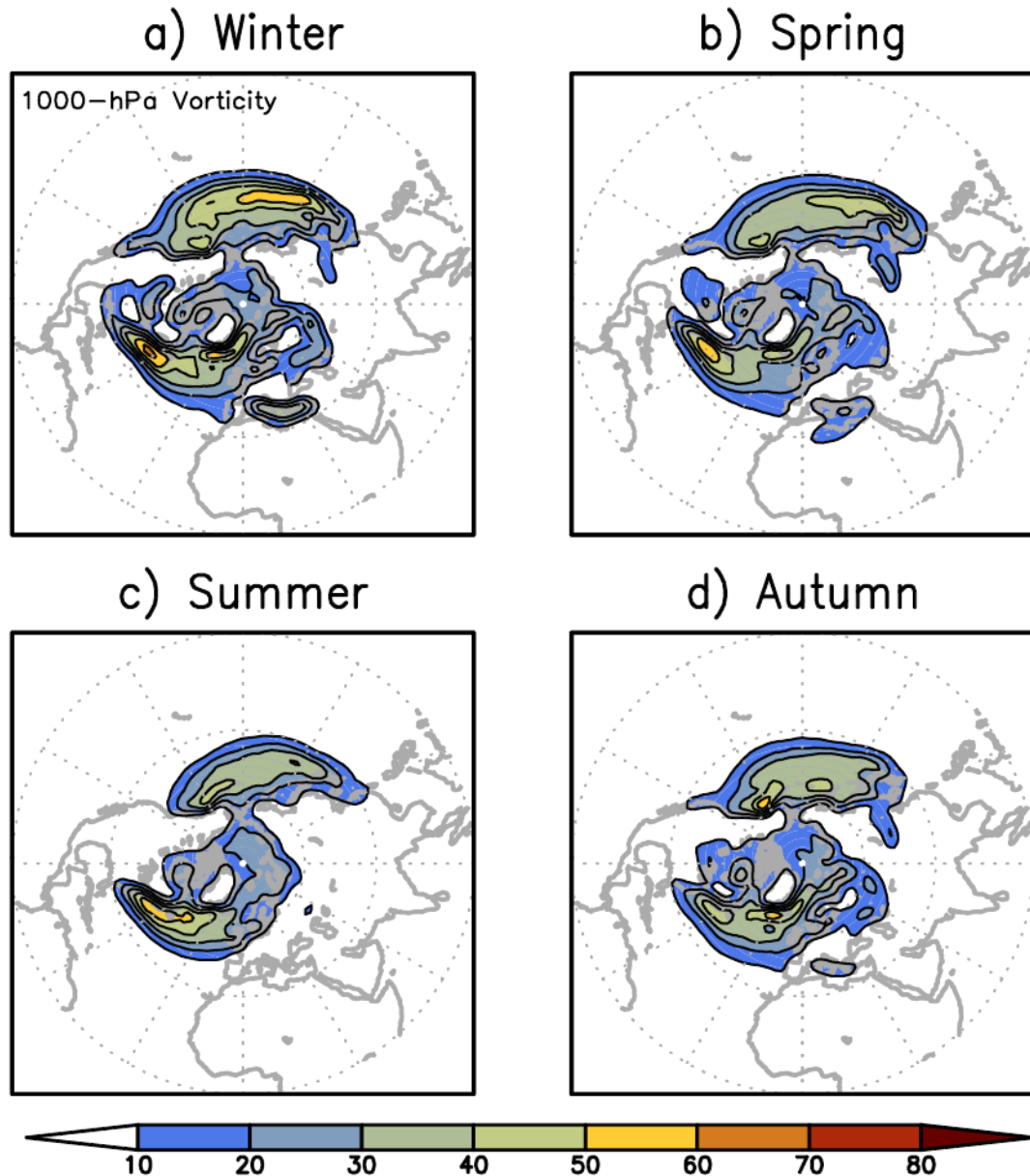
Figure 2: Track density for positive 1000-hPa relative vorticity for boreal seasons for the period (1979-2014): a) Winter, b) Spring, c) Summer and d) Autumn. Units are number density per season per unit area where unit area is equivalent to 5^\circ radius spherical cap.
