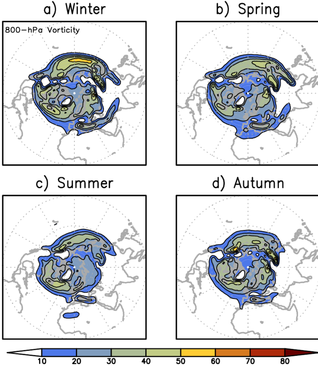
Figure 3: Track density for positive 800-hPa relative vorticity for boreal seasons for the period (1979-2014): a) Winter, b) Spring, c) Summer and d) Autumn. Units are number density per season per unit area where unit area is equivalent to 5^\circ radius spherical cap.
