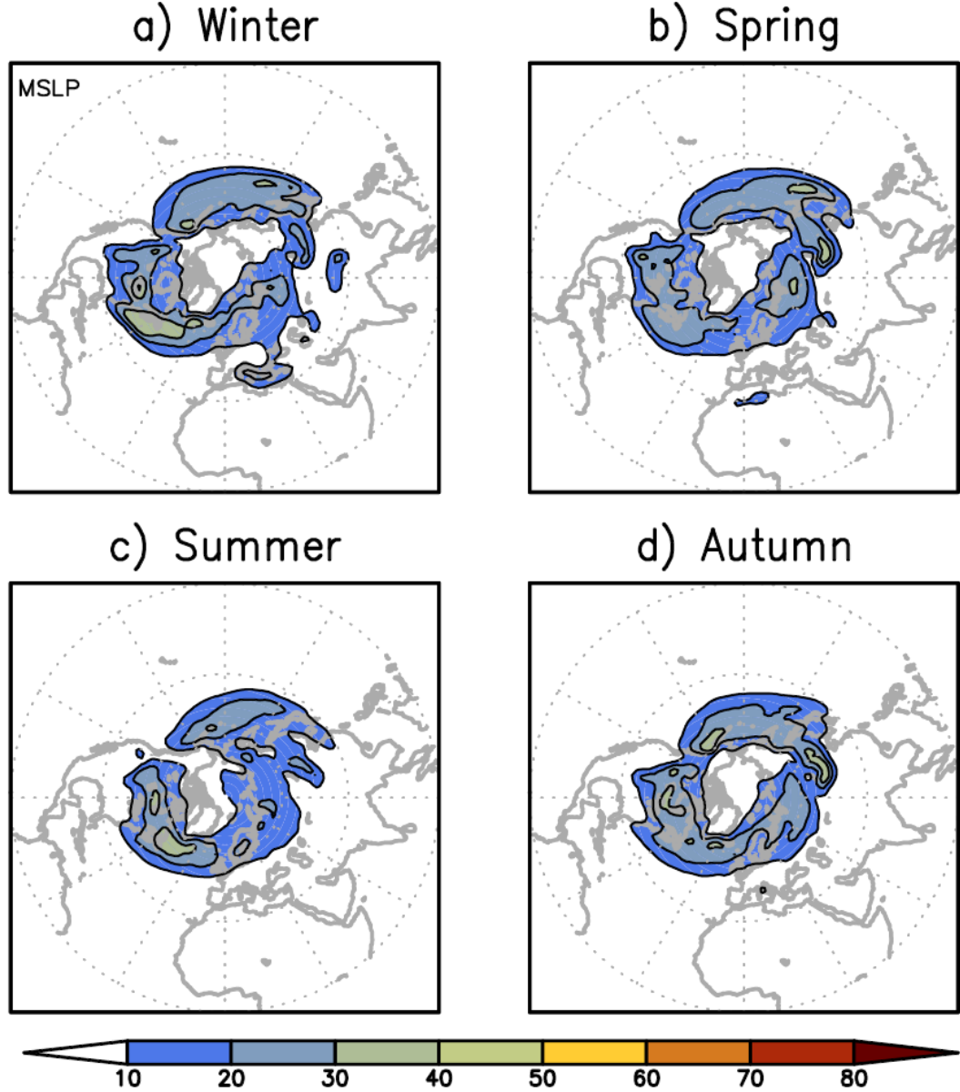
Figure 1: Track density for negative MSLP (seasonal mean) for boreal seasons for the period (1979-2014): a) Winter, b) Spring, c) Summer and d) Autumn. Units are number density per season per unit area where unit area is equivalent to 5^\circ radius spherical cap.
