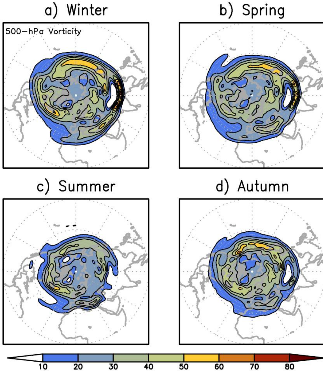
Figure 4: Track density for positive 500-hPa relative vorticity for boreal seasons for the period (1979-2014): a) Winter, b) Spring, c) Summer and d) Autumn. Units are number density per season per unit area where unit area is equivalent to 5^\circ radius spherical cap.
