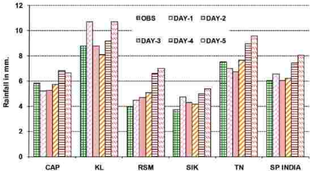
Seasonal Mean Rainfall (mm) :NE Monsoon 2010
