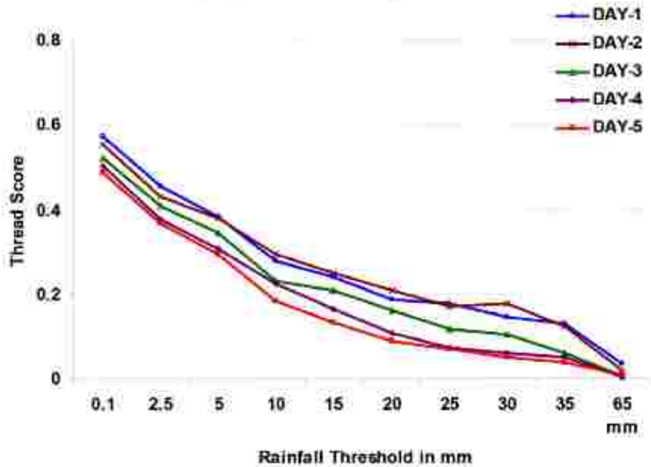
Fig.8 The Thread Score (TS) between daily domain mean observed and forecasted precipitation of day-1 to day-5 for southern Peninsular India during 1 October -31 December 2010.
